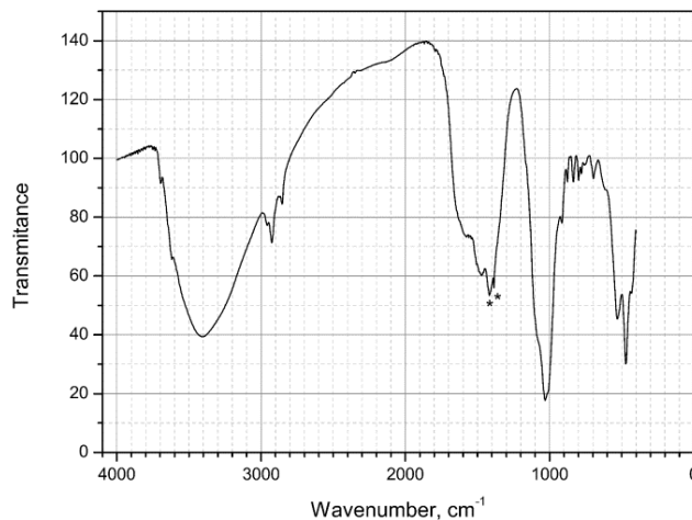
Figure 3. Results of FTIR analysis of deposits on inner side of condenser tube near fracture site. Wave-number peak at 1417 cm⁻¹ corresponds to ammonia compounds, while wave-number peak of 1385 cm⁻¹ corresponds to nitrate compounds.
