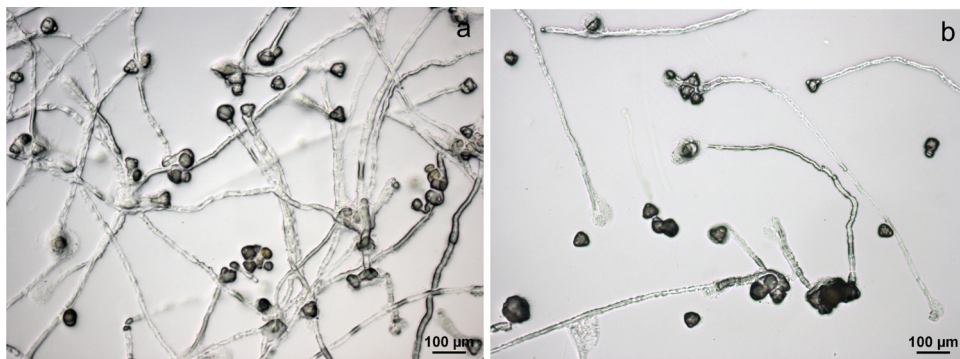
Fig. 5. Pollen germination.
