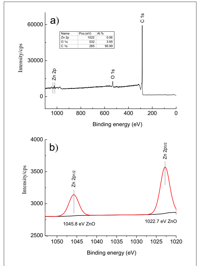
Fig. 8. The XPS Spectra Taken from the Zn/GAC Sample: a) the survey spectrum showing the position and the atomic percentage of the main components; b) the high resolution region spectrum of Zn 2p showing the fitted binding energies.
