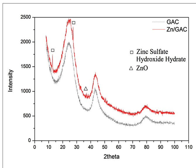
Fig. 4. XRD Pattern of GAC (Dotted-line) and the Zn/GAC Sorbent (Solid-line).
