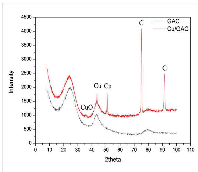
Fig. 3. XRD Patterns of GAC (Dotted-line) and the Cu/GAC Sorbent (Solid-line).
