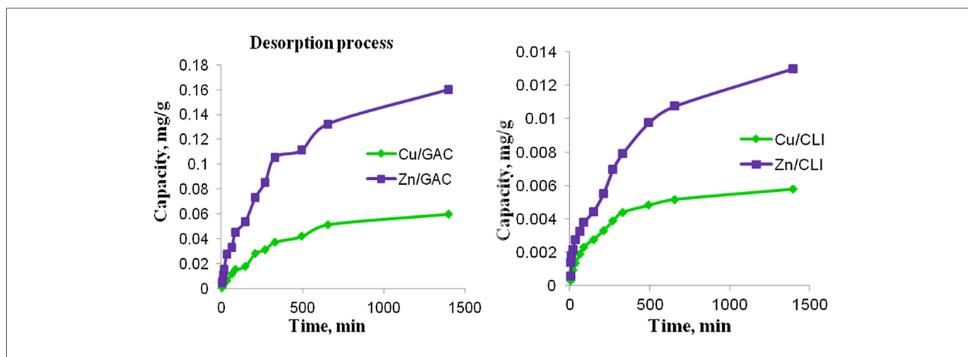
Fig. 2. Desorption of \text{Cu}^{2+} and \text{Zn}^{2+} ions from the Cu/GAC, Zn/GAC, Cu/CLI and Zn/CLI Sorbents.
