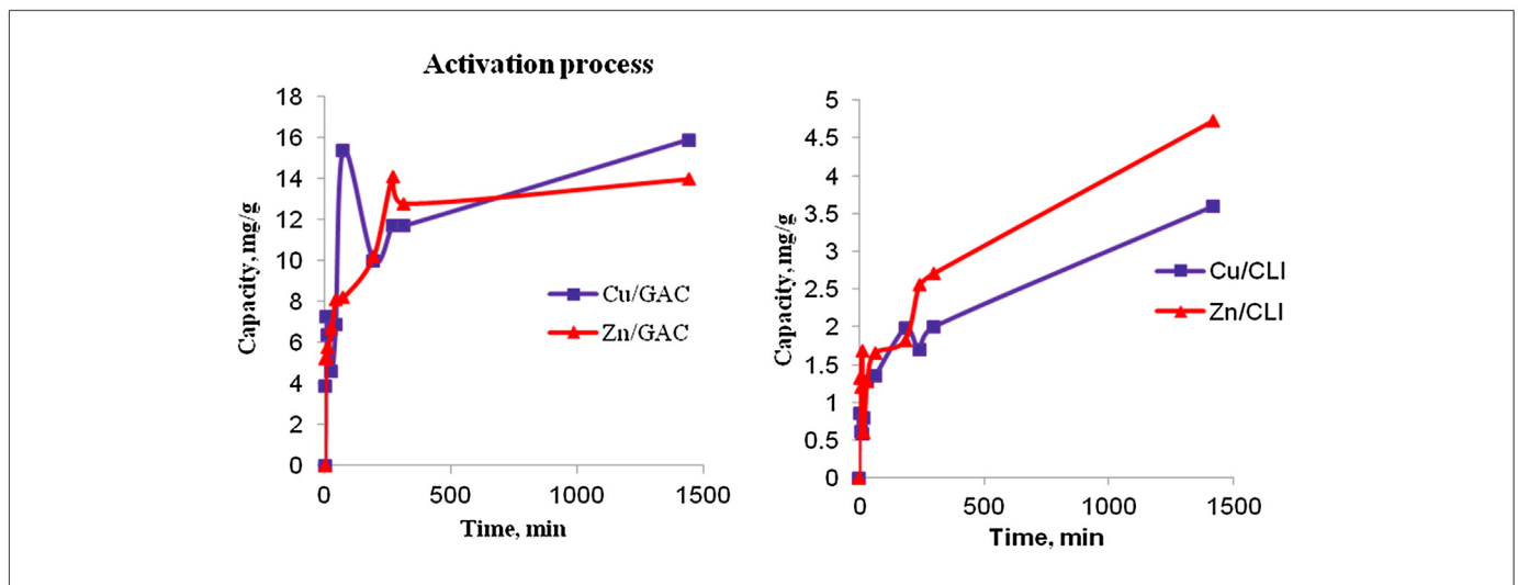
Fig. 1. Activation Process of Gac and Cli Sorbents by Cu 2+ and Zn 2+ ions.
