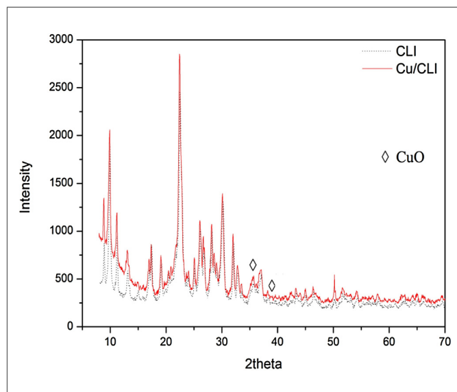
Fig. 5. XRD Patterns of CLI (Dotted-line) and the Cu/CLI Sorbent (Solid-line).
