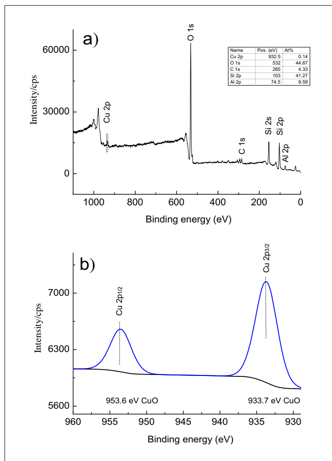
Fig. 9. The XPS Spectra Taken from the Cu/CLI Sample: a) the survey spectrum showing the position and the atomic percentage of the main components; b) the high resolution region spectrum of Cu 2p showing the fitted binding energies.
