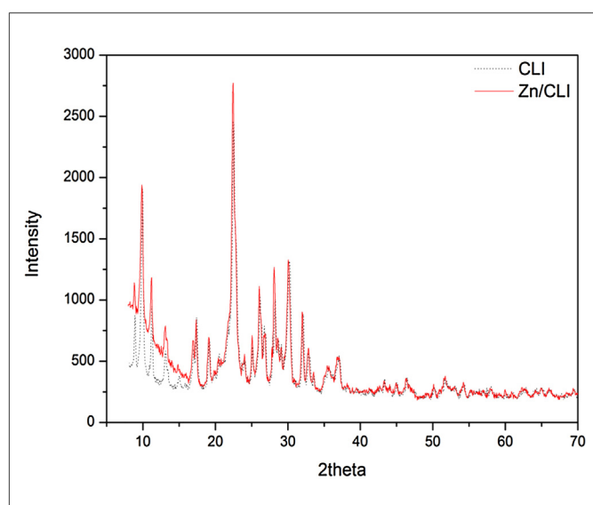
Fig. 6. XRD Patterns of CLI (Dotted-line) and the Zn/CLI Sorbent (Solid-line).
