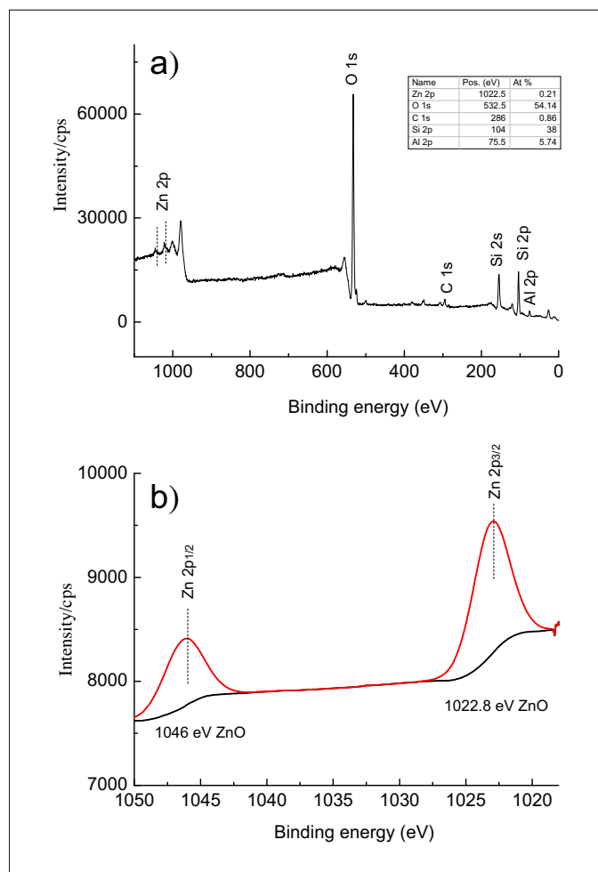
Fig. 10. The XPS Spectra Taken from the Zn/CLI Sample: a) the survey spectrum showing the position and the atomic percentage of the main components; b) the high resolution region spectrum of Zn 2p showing the fitted binding energies.
