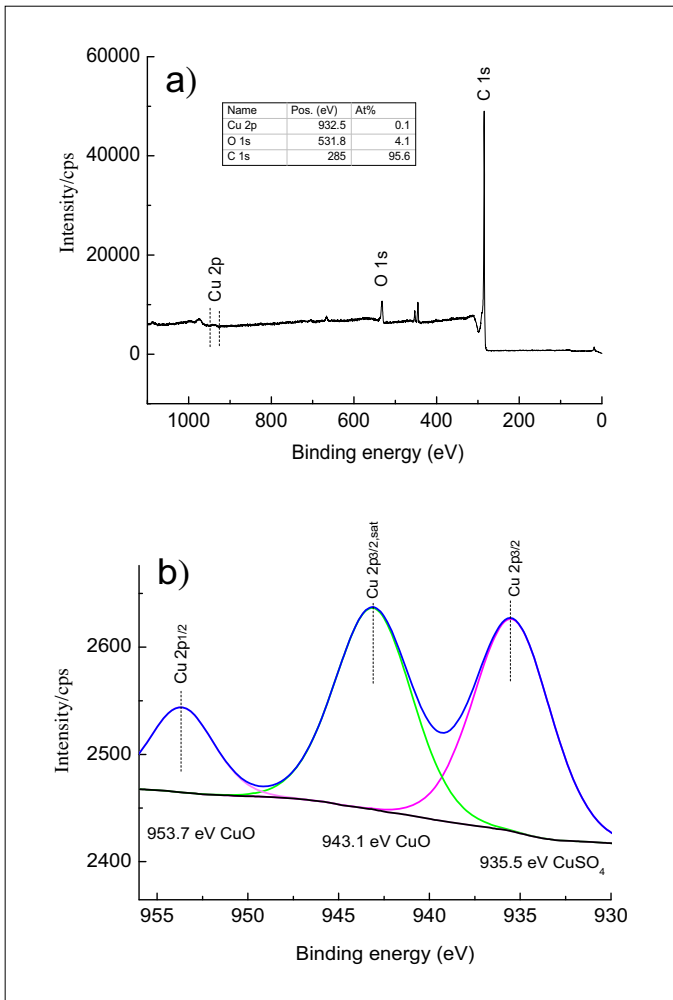
Fig. 7. XPS Spectra Taken from the Cu/GAC Sample: a) the survey spectrum showing the position and the atomic percentage of the main components; b) the high resolution region spectrum of Cu 2p showing the fitted binding energies.
