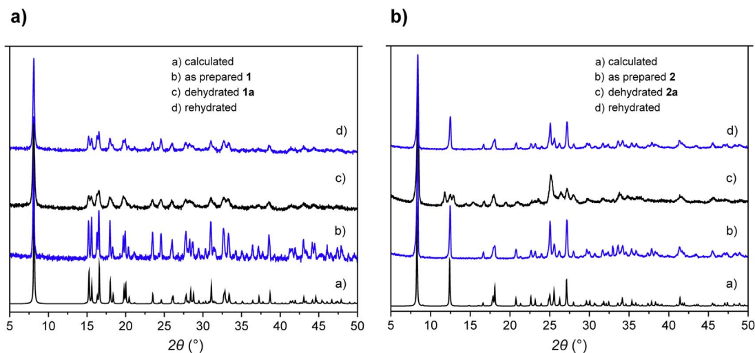
Fig. 5. XRPD patterns of: a) 1 b) 2.
