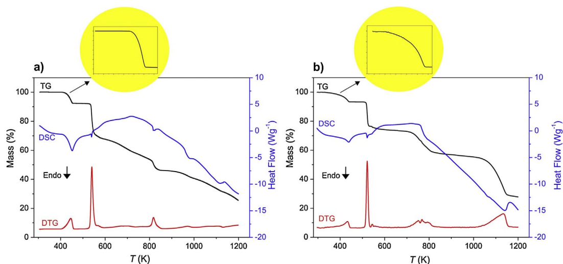
Fig. 1. Simultaneous TG-DSC-DTG plots at \beta = 20 \text{ K min}^{-1} in a nitrogen atmosphere of: a) 1 b) 2.
