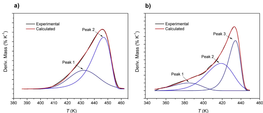
Fig. 7. Deconvolution of complex dehydration process at \beta = 20 \text{ K min}^{-1} : a) for 1 b) for 2.
