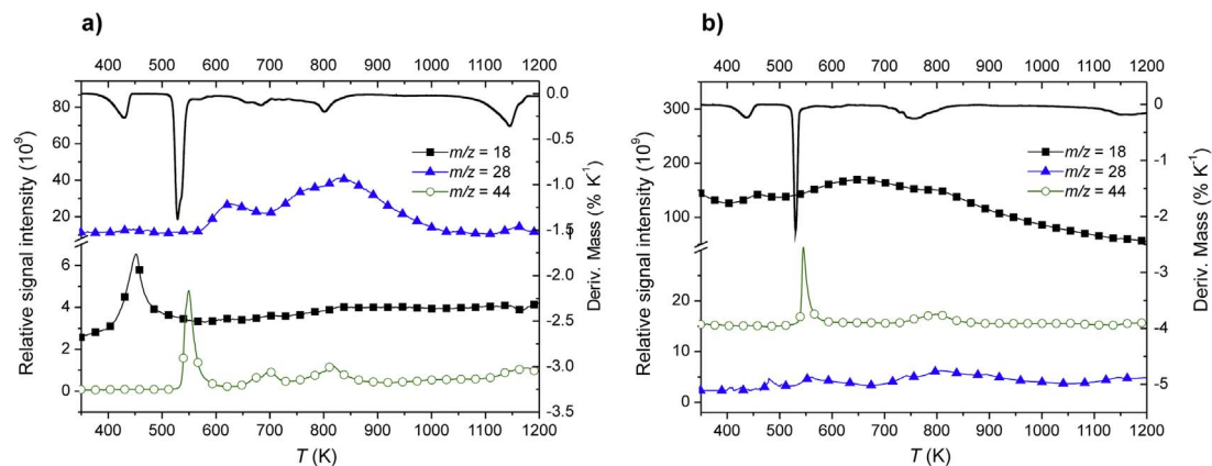
Fig. 2. TG/MS data for dehydration and decarboxylation in argon atmosphere of: a) 1 b) 2.
