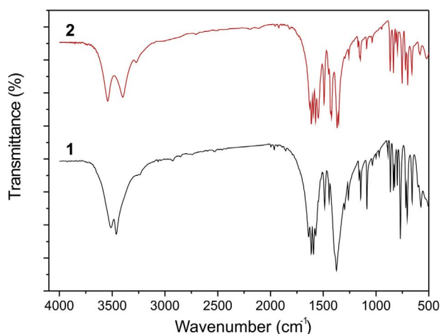
Fig. 4. FT-IR spectra of 1 and 2.
