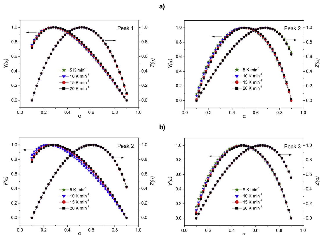
Fig. 9. Målek curves y(\alpha) and z(\alpha) at different heating rates, determined for dehydration: a) 1 b) 2.
