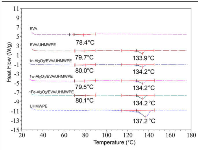
Figure 7. DSC thermograms of EVA, UHMWPE fibres and composite fibres.
