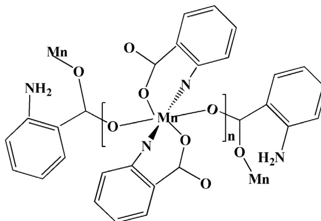
Scheme 1 Schematic representations of the coordination modes for the carboxylate bridges.
