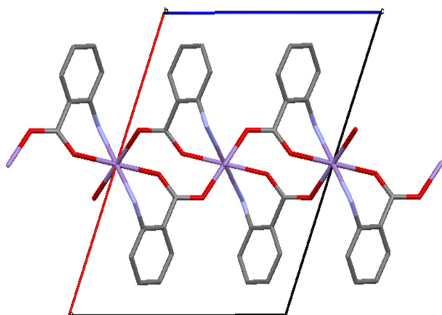
Figure 2 View of the coordination environment around Mn(ii).
