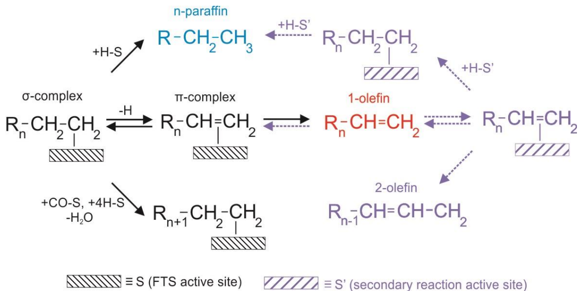
Figure 2.6 – Schematic of primary FTS and secondary olefin reactions
