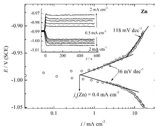
Fig. 2. Polarization curve ( v = 1 \text{ mV s}^{-1} ) of the zinc electrode in 2 \text{ M NH}_4\text{Cl} and 1.1 \text{ M ZnCl}_2 .
