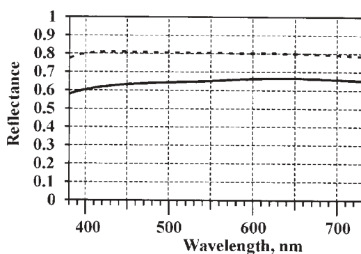
Fig. 1. Dependence of the reflection on wavelength: ( - - ) specimen A-1; (—) specimen A-4.
