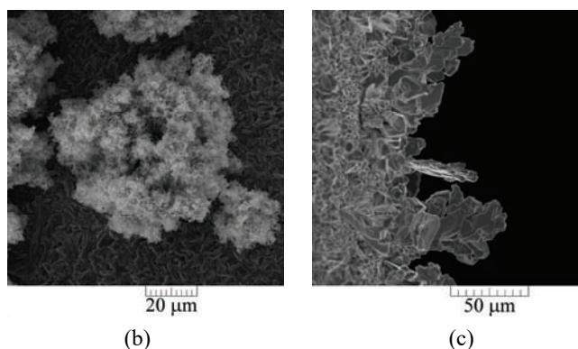
Fig. 7. a) The polarization curve for Zn electrodeposition from 0.10 M ZnSO 4 in 2.0 M NaOH, and the typical surface morphologies obtained at overpotentials of: b) \eta = 45 mV (zone of the rapid increase in the current density with increasing overpotential), t = 60 min, and c) \eta = 100 mV (plateau of the limiting diffusion current density), t = 50 min.
