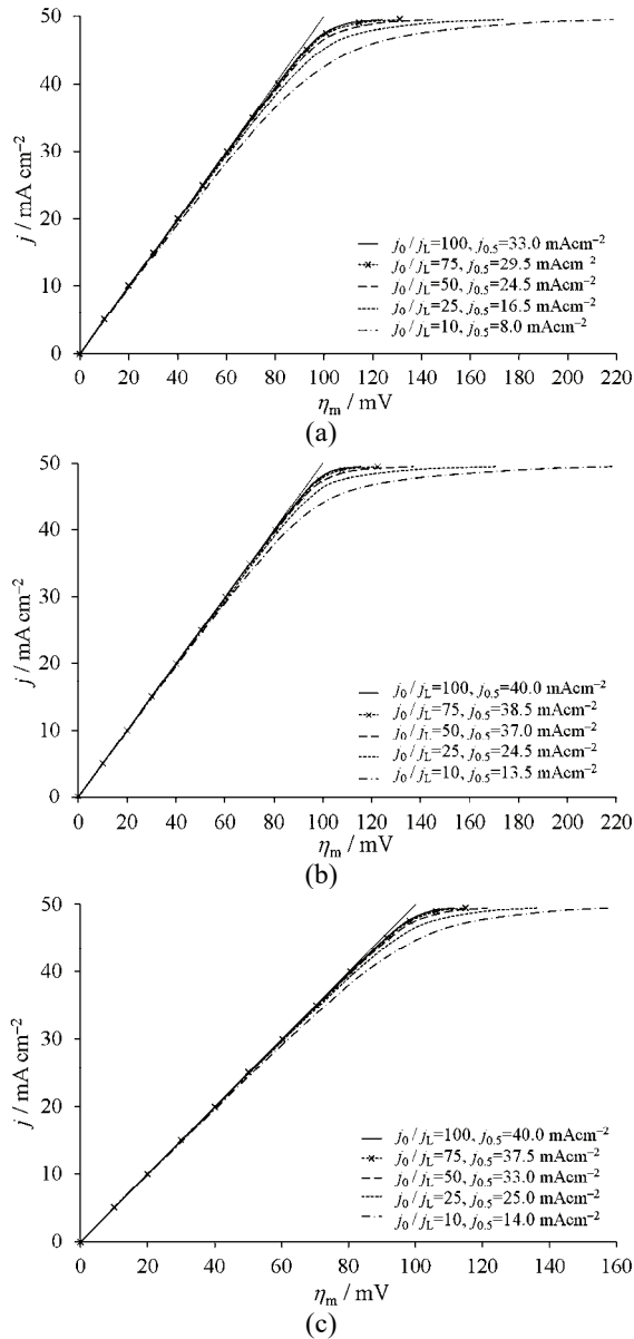
Fig. 3. Dependencies j-\eta_m for 10 \leq j_0/j_L \leq 100 calculated as those in Fig. 2; a), b) and c) as in the captions in Fig. 1; d) the manner for the determination of j_{0,5} .
