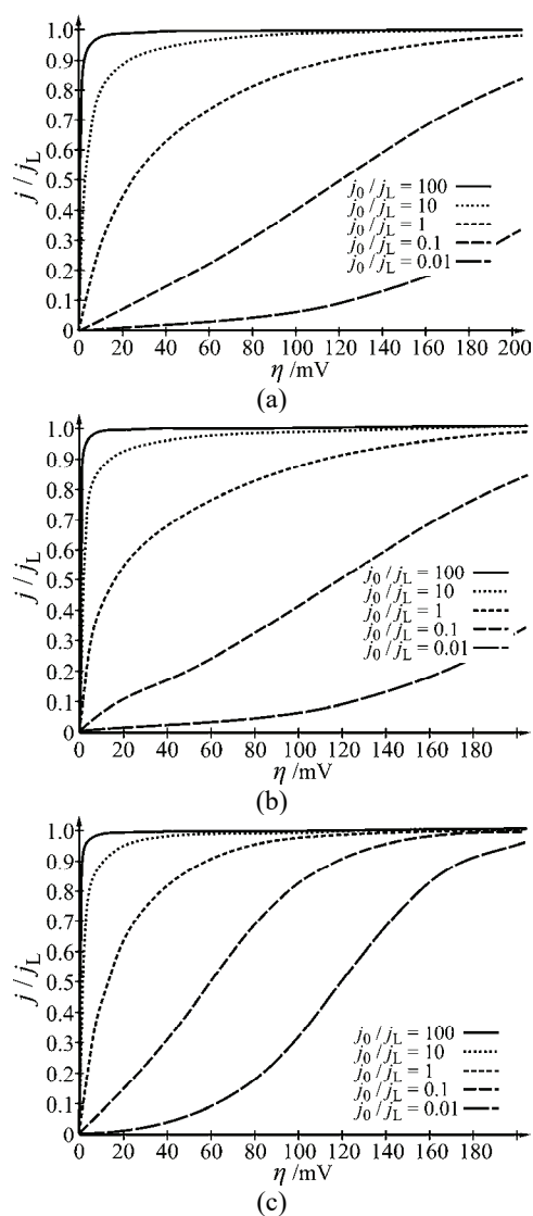
Fig. 1. Dependencies j/j_L-\eta calculated using Eqs. (2) and (3) for different values of the j_0/j_L ratio: a) b_a = 120 \text{ mV dec}^{-1} , b_c = 120 \text{ mV dec}^{-1} , b) b_a = 40 \text{ mV dec}^{-1} , b_c = 120 \text{ mV dec}^{-1} and c) b_a = 60 \text{ mV dec}^{-1} , b_c = 60 \text{ mV dec}^{-1} .
