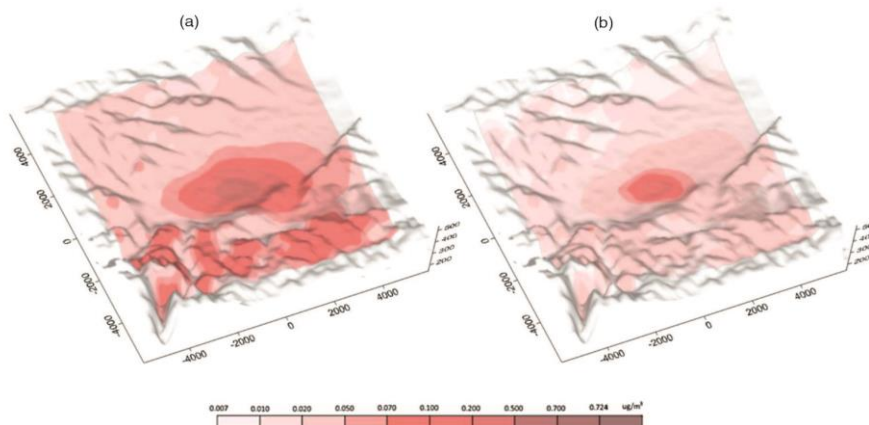
Figure 4. The TPM ground level distribution emitted by (a) fuel oil-fuelled boiler and (b) natural gas-fuelled boiler
