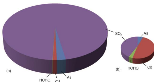
Figure 5. Hazard index contributions of the various pollutants emitted by; (a) fuel oil boiler and (b) natural gas boiler
