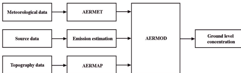
Figure 2. Flow chart showing the AERMOD workflow with the respective input and output pathways
