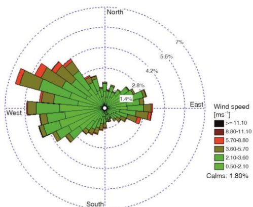
Figure 3. Valjevo wind rose
