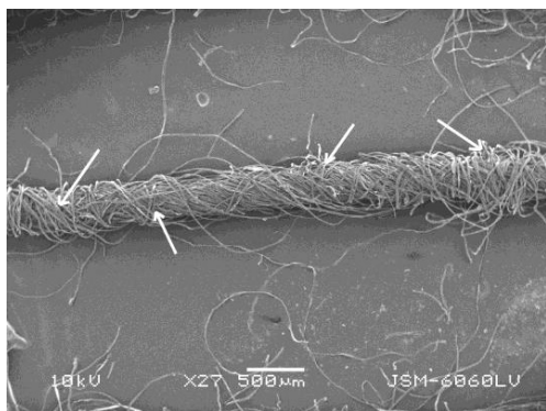
Figure 1. The SEM illustrating structure of cotton OE yarn designated as Co3 (the highest twist level)
