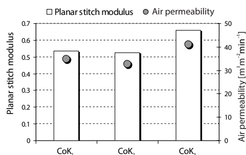
Figure 3. Planar stitch modulus and air permeability of the knitted fabrics
