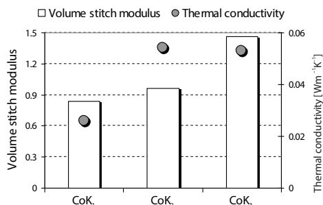
Figure 4. Volume stitch modulus and thermal conductivity of the knitted fabrics
