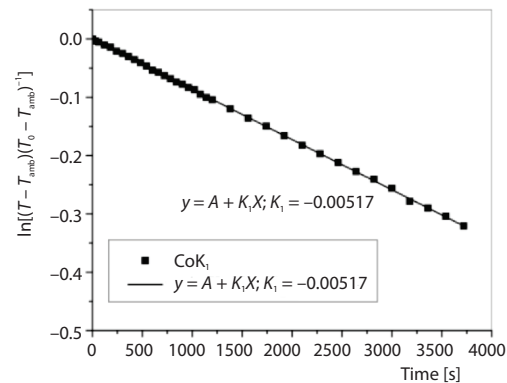
Figure 2. Cooling line and cooling constant, K_1 , of the CoK 1 knitted fabric
