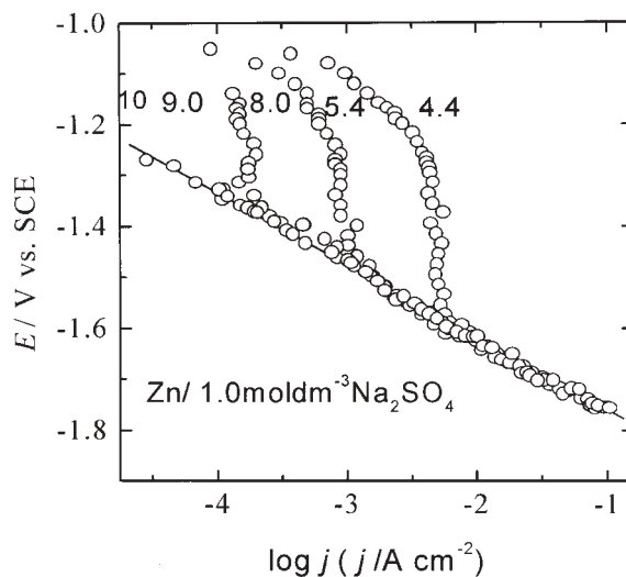
Fig. 1. Tafel polarization curves for the her on a Zn electrode in 1.0 \text{ mol dm}^{-3} \text{ Na}_2\text{SO}_4 solutions of different pH values at 25.0 °C.
