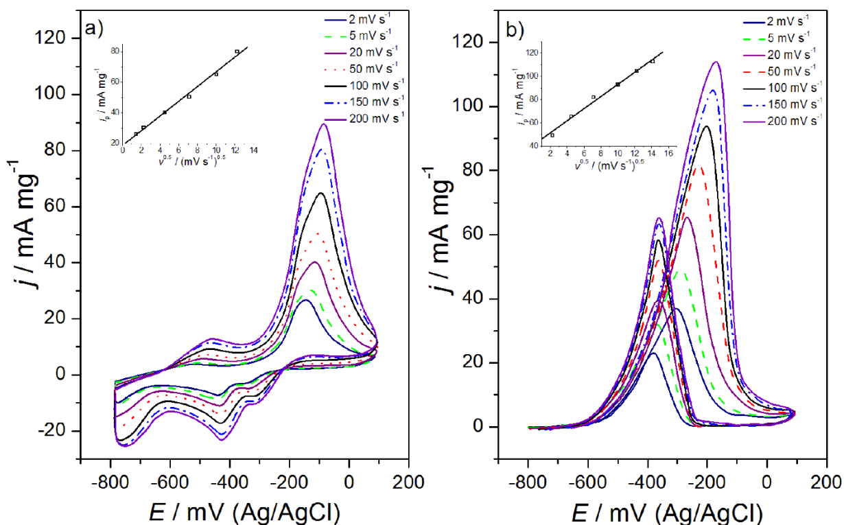
Fig. 8. CVs of (a) Pd and (b) Sn (-1800 mV) -Pd electrocatalysts in 1 M NaOH + 1 M C 2 H 5 OH solution recorded at v = 2, 5, 20, 50, 100, 150, and 200 \text{ mV s}^{-1} . Inset: dependency of j_p from v^{0.5}
