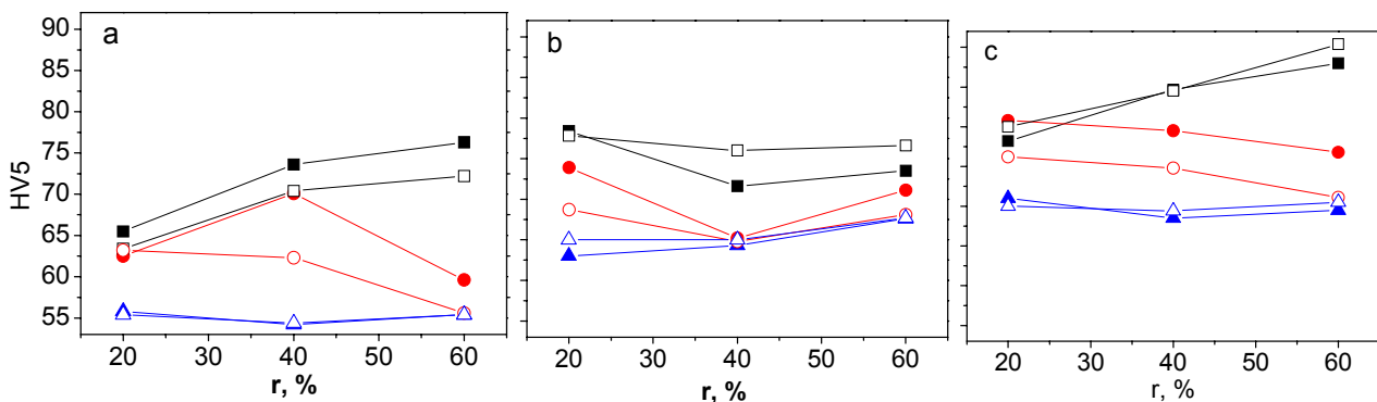
Fig. 8. The influence of cold rolling reduction on hardness after annealing for 3 hours at: ■-250°C, ●-280°C, ▲-350°C, slow heating-closed symbols; rapid heating –opened symbols; (a) AlMg3, (b) AlMg4.5Mn and (c) AlMg6Mn.
