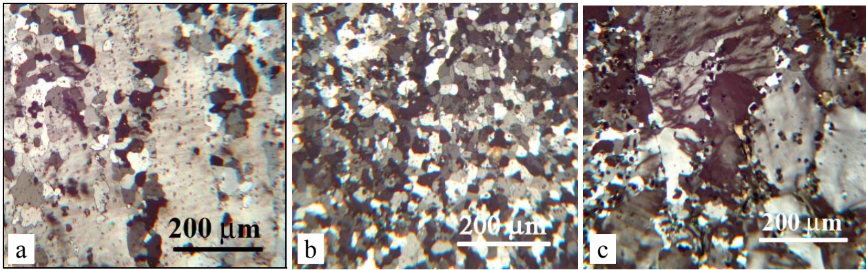
Fig. 6. Microstructures of (a) AlMg3, (b) AlMg4.5Mn and (c) AlMg6Mn after 40% cold rolling followed by annealing at 280°C for 3 hours; rapid heating.
