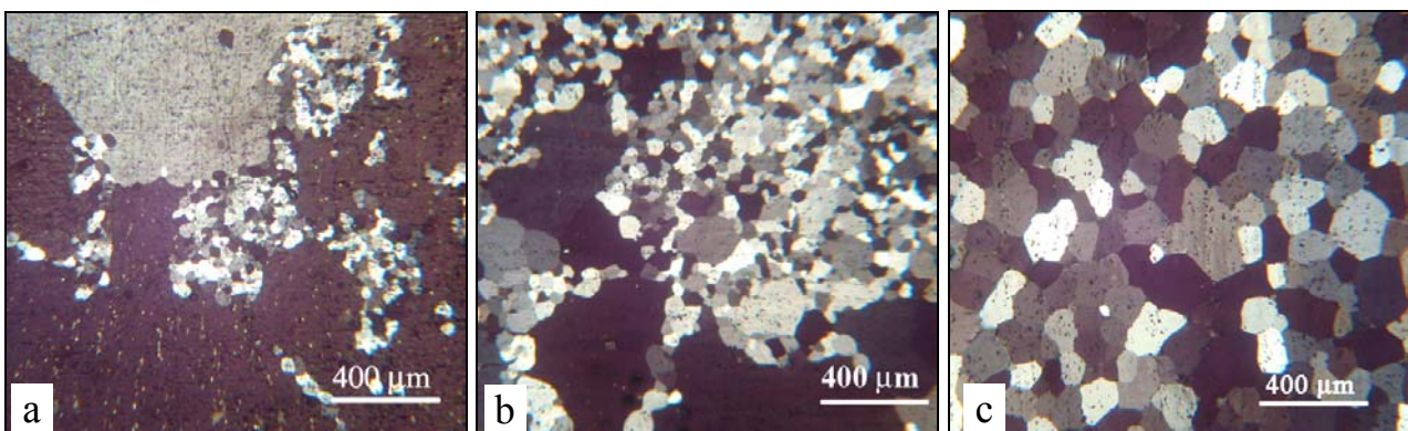
Fig. 1. Grain structure after two-stage annealing of the AlMg3 (a), AlMg4.5Mn (b) and AlMg6Mn (c) alloy sheets.
