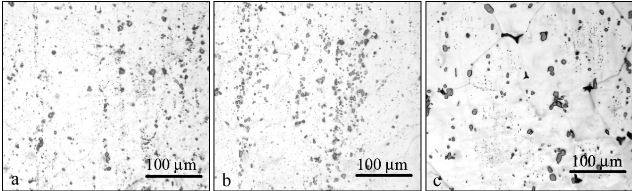
Fig. 2. Particle distribution in the tested alloys after two-stage annealing: (a) AlMg3, (b) AlMg4.5Mn and (c) AlMg6Mn.
