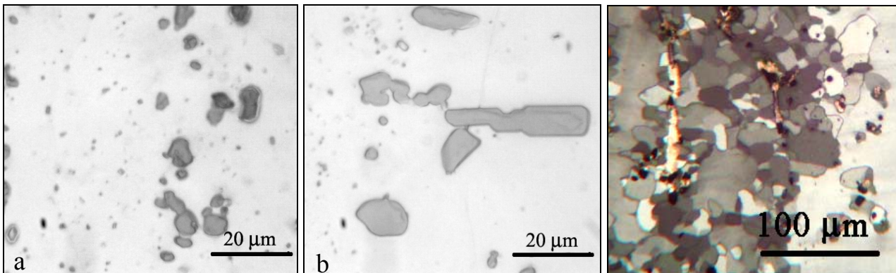
Fig. 4. Particles in the tested alloys after two-stage annealing: (a) AlMg4,5Mn and (b) AlMg6Mn
