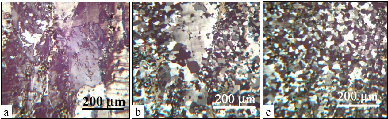
Fig. 3. Microstructures in AlMg6Mn alloy after 60% reduction and annealing at: (a) 250°C/3h, (b) 280°C/3h and (c) 350°C/3h; rapid heating.
