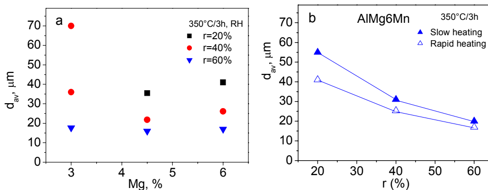
Fig. 7. The influence of (a) Mg content and (b) cold rolling reduction and heating rate, on recrystallized grain sizes.
