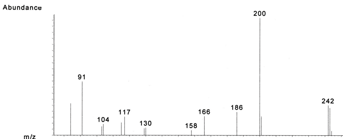
Slika 15. Maseni spektar PCP. Figure 15. Mass spectra of PCP.
