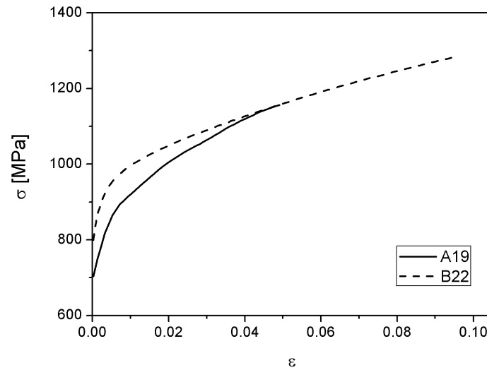
Figure 3. Tensile true stress – true strain curves at 77 K.
