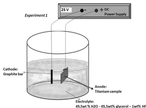
Fig. 1. Schematic overview of the anodizing process [11].
