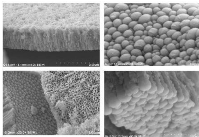
Fig. 2. SEM micrographs of nanotubular layer formed at 25 V during 180 min long anodization process [32].
