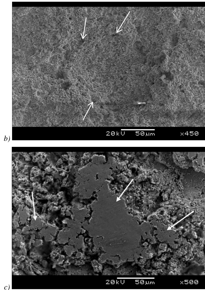
Fig. 3. SEM micrographs of the damaged surface of hot-pressed samples: a) CuHP, b) 5hHP-L, and c) 30hHP-H, after 120 min of cavitation erosion testing.
