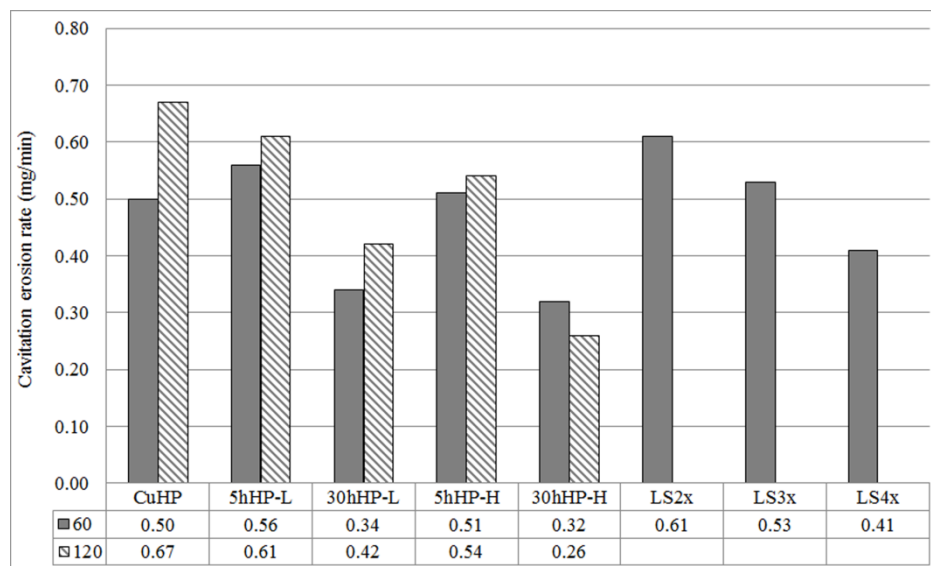
Fig. 2. Cavitation erosion rates of hot-pressed and laser-sintered samples.
