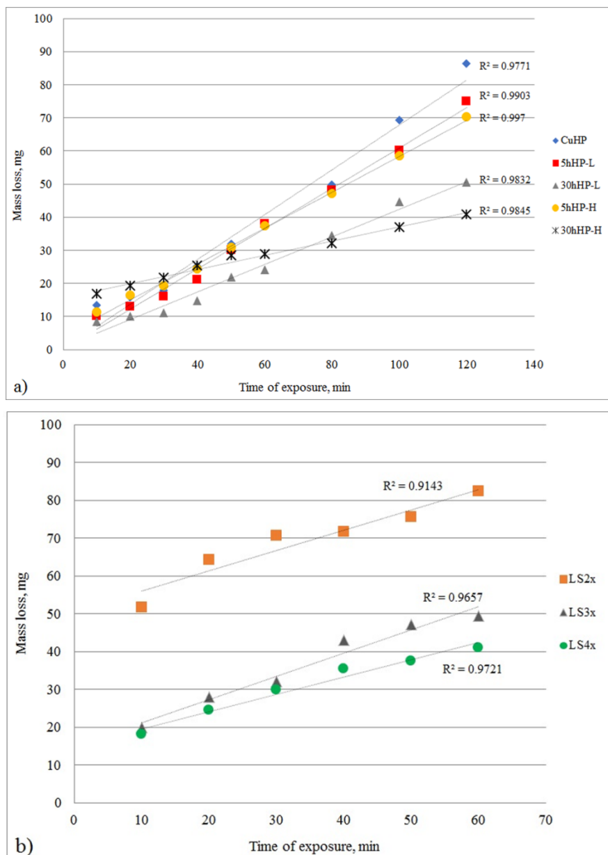
Fig. 1. Mass loss during cavitation erosion testing of a) hot-pressed and b) laser-sintered samples.
