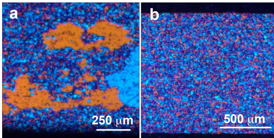
Fig. 4. OM. (a) The microstructure of the alloy C after 85 % cold reduction and annealing 1 h at 480 °C; (b) microstructure of the alloy D after 85 % cold reduction and annealing 1 h at 520 °C.
