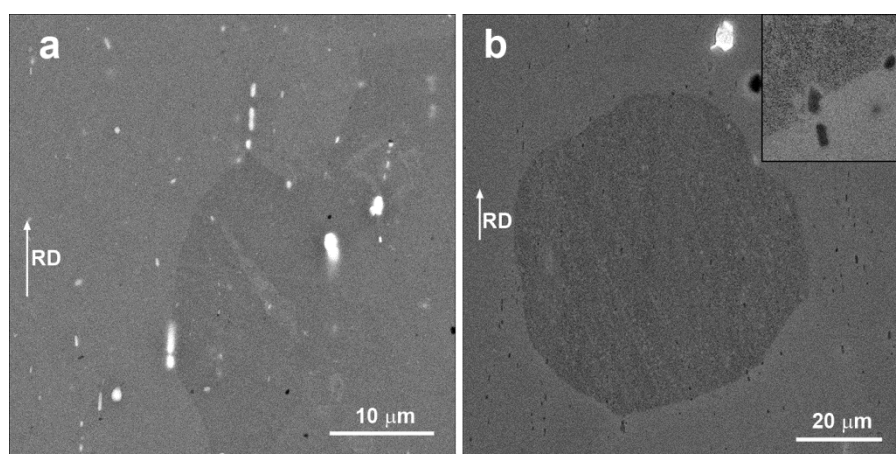
Fig. 3 (a) SEM micrograph of the rod-like Al_6Mn(Fe) particles at the grain boundaries. The micrograph is of the boundary between two abnormal grains in the alloy A after annealing at 480 °C for 1 h. (b) SEM micrograph of the island grain within the abnormal grain in the alloy A. Insert shows the pinning of the boundary by dispersoids. The specimen was etched by Barker's reagent after annealing at 520 °C for 1 h.
