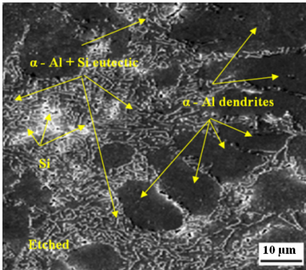
Figure 7: (SEM) Etched microstructure of the Al-12Si coating: \alpha -Al dendrites, \alpha -Al + Si
