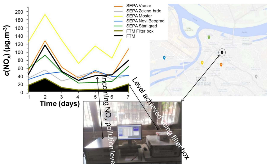
Figure 34. Evidence of reaching air quality better than the lowest measured in the low traffic density suburbs of Belgrade, Serbia. \text{NO}_x concentration recordings in ambient air for five sampling points in the city of Belgrade in relation to the FTM sampling points (1 d mean values from 13 to 19 October 2019) [40,41].
