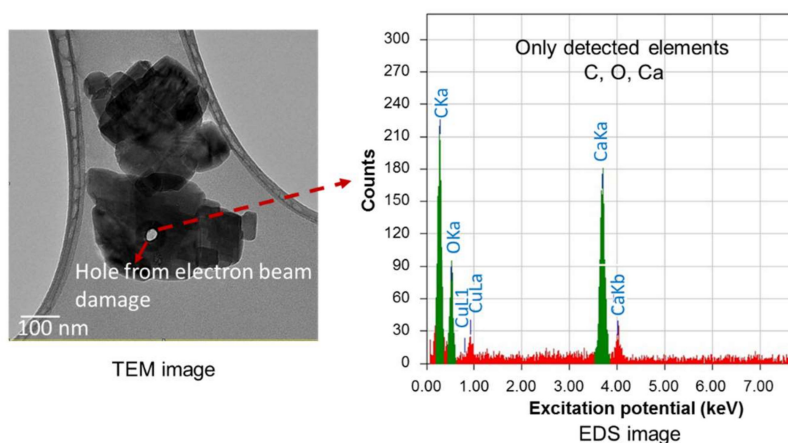
EDS spectrum from scraped coating powder (GCC + MNFC): H 2 O 2 pre-oxidised non-exposed
