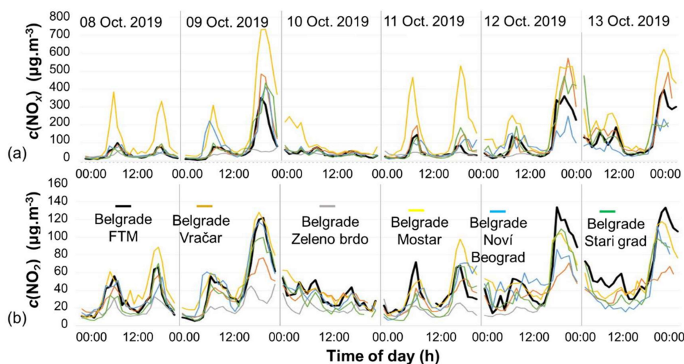
Figure 18. Monitoring of (a) total NO x and (b) NO 2 levels to compare official data from a range of monitoring stations with laboratory sampling of external air at the Faculty of Technology and Metallurgy (FTM), Belgrade (1-h mean values).
