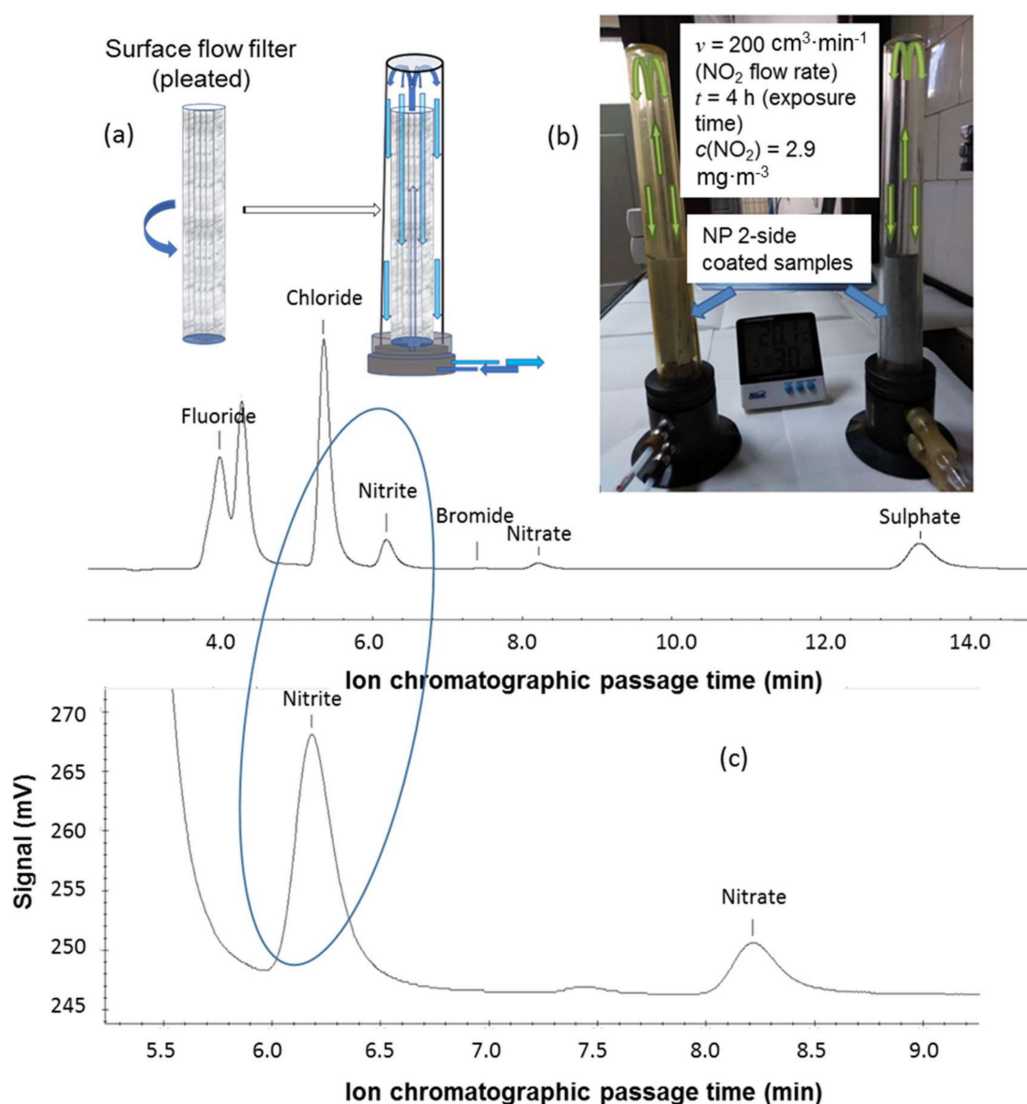
Figure 17. (a) Schematic of the flow system that shows inlet and filter-contact outlet flows, (b) the samples (smooth two-side coated recycled newspaper substrate (NP)) mounted in practice—gas concentration is shown as c(\text{NO}_2) = 2.9 \text{ mg} \cdot \text{m}^{-3} , and (c) ion chromatograph that shows the predominance of nitrite on a pre-wetted sample.
