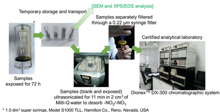
Figure 13. Static exposure procedure for coated samples, which included the gas-loaded super syringe, removed samples in storage vessels and aqueous extraction for ion chromatographic analysis.
