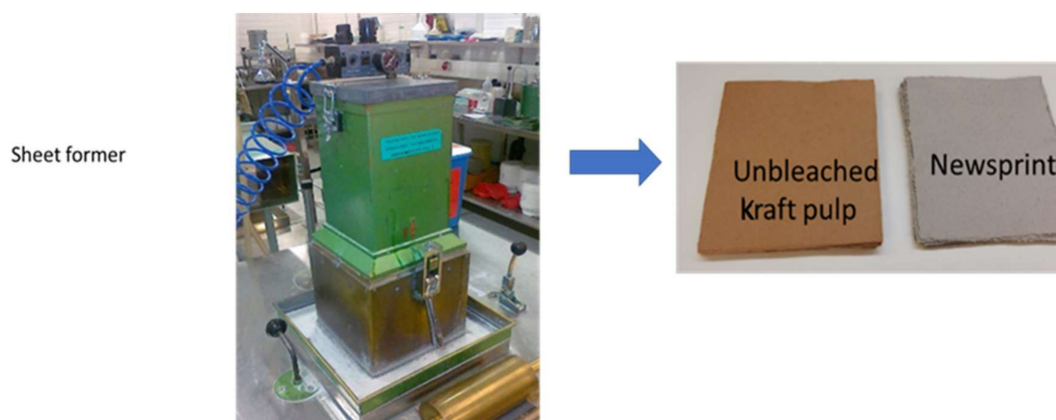
Figure 5. Sheet-forming the substrate sheets using a laboratory hand sheet former. The examples shown were made from unbleached Kraft (brown) and from the recycled newsprint (grey).
