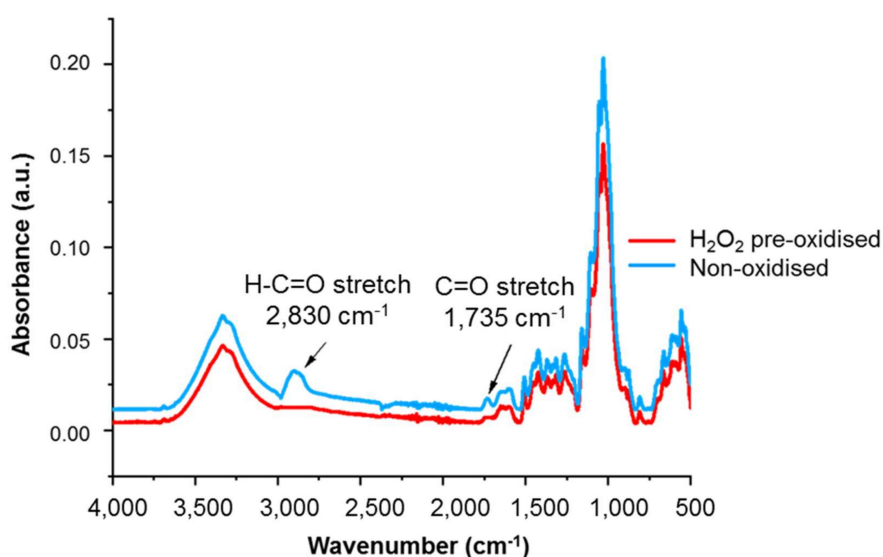
Figure 25. The Fourier transform infrared (FTIR) spectral analysis of recycled newsprint substrate that illustrates the action of pre-oxidation by removing the \text{H}-\text{C}=\text{O} stretch band.
