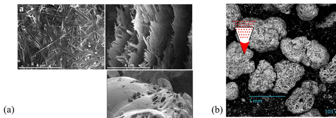
Fused perlite and its illustrative action of pore condensation
