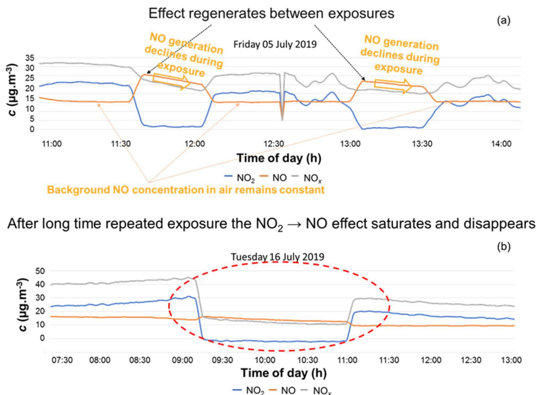
Figure 23. (a) Regeneration of the NO 2 → NO effect between exposures while background NO level in the incoming air is constant, (b) long time repeated exposure (as shown Friday 5th July–Tuesday 16th July 2019) saturates the RedOx reaction.
