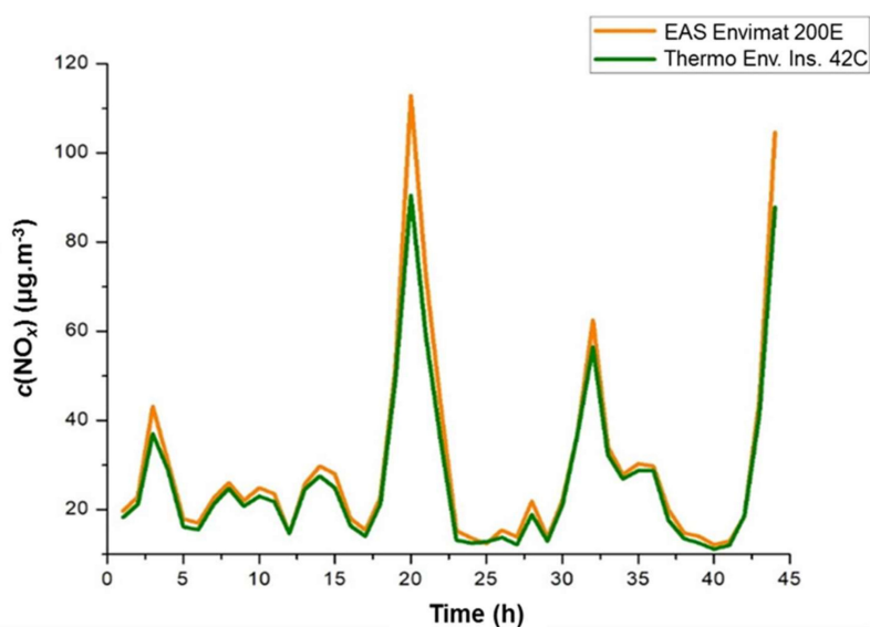
Figure 19. Comparison of ambient NO x concentrations (Faculty of Technology and Metallurgy (FTM), University of Belgrade, sampling point) between chemiluminescence NO-NO 2 -NO x analysers: Thermo Environmental Instruments 42C (green line) vs. EAS Envimet ČR, č.r.o. 200E (orange line).
