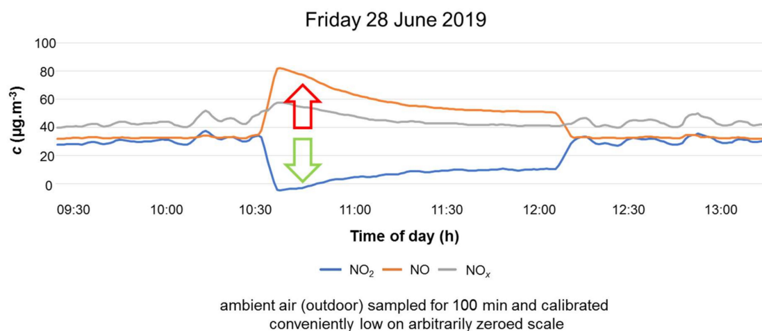
Figure 22. Insertion of the box design surface flow filter in the stream of externally sampled air. The red arrow indicates the generation of \text{NO} while the green arrow indicates \text{NO}_2 concentration and drops during the period of exposure.
