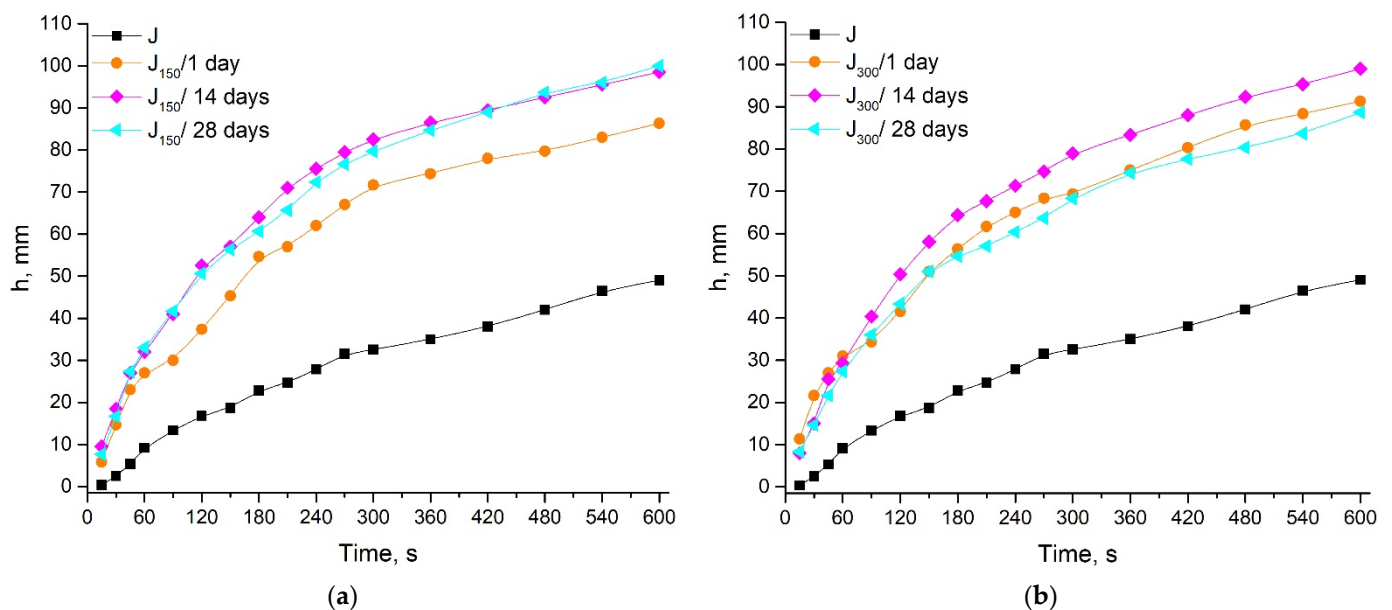
Figure 7. Effect of aging on the capillary rise height ( h ) of plasma-treated jute fabrics at (a) 150 Hz and (b) 300 Hz.
