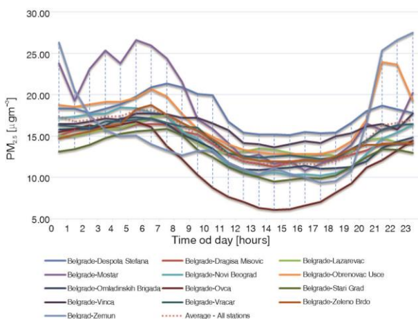
Figure 2. Average hourly PM 2.5 concentrations at the air monitoring stations (for color image see journal web site)
