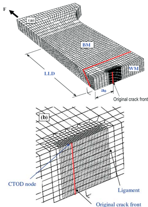
Figure 3 Three-dimensional finite element model for CCT specimen. (a) 3D finite element mesh for one eighth of specimen. (b) Detailed mesh for the region near the crack front
