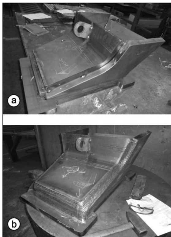
Figure 2 The connection part of the transporter's construction during manufacturing, a) before welding, b) after welding
