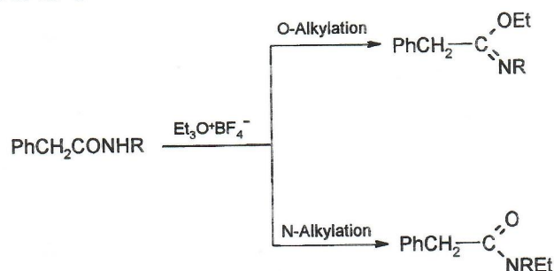
Scheme 6. Alkylation of N-substituted 2-phenylacetamides with triethyloxonium tetrafluoroborate.
