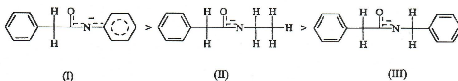
Scheme 9. The order of reactivity – structure of the formed anions of PPA (I), EPA (II) and BPA (III).
