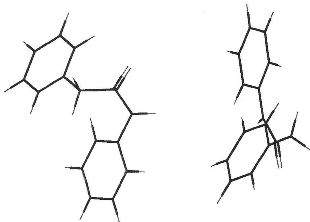
Fig. 5. Two views of the most stable conformation of PPA showing the susceptibility to base attack on either the hydrogen on the nitrogen atom or the hydrogen(s) on the \alpha_{C=O} -carbon atoms.
