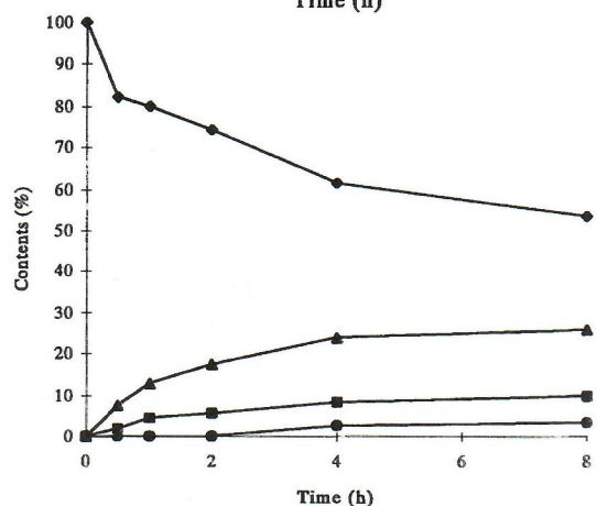
Fig. 4. Alkylation of EPA with benzyl chloride at reflux temperature in the presence of KOH in toluene (equimolar amounts of reactants; \blacklozenge – EPA; \blacksquare – C-product; \blacktriangle – N-product; \bullet – C,N-product).
