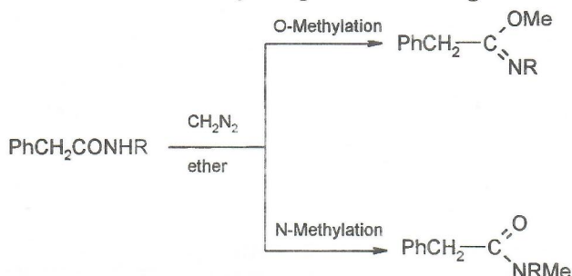
Scheme 1. Alkylation of N-substituted 2-phenylacetamides with ethereal diazomethane solution.
