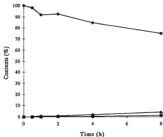
Fig. 3. Alkylation of EPA with benzyl chloride at 60 °C in the presence of KOH in toluene (equimolar amounts of reactants; \blacklozenge – EPA, \blacksquare – C-product; \blacktriangle – N-product).
