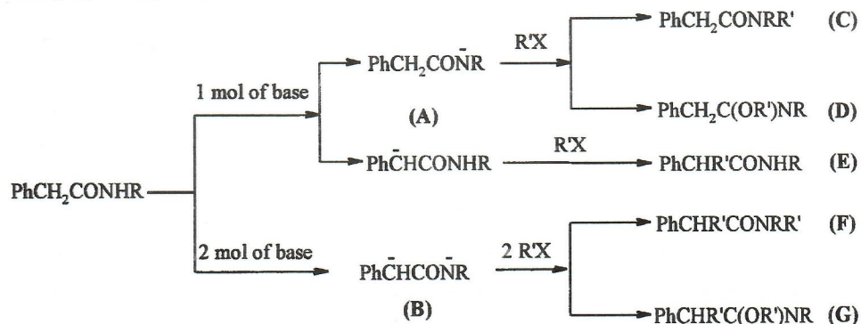
Scheme 10. PTC extraction mechanism for the alkylation of N-substituted phenylacetamides. 24
