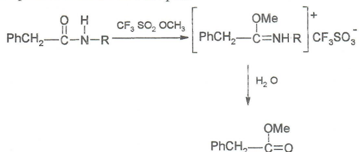
Scheme 7. Alkylation of N-substituted 2-phenylacetamides with methyl trifluoromethanesulfonate.
