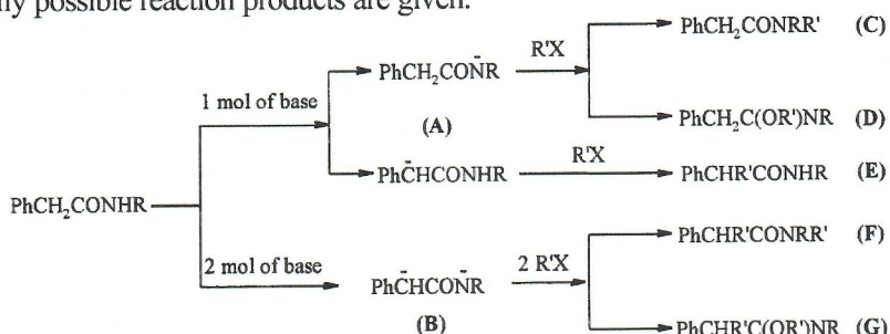
Scheme 8. Alkylation of N-substituted 2-phenylacetamides under basic conditions ((A)-monoanions, (B)-dianion, (C)-N-product, (D)-O-product, (E)-C-product, (F)-C,N-product, (G)-C,O-product).
