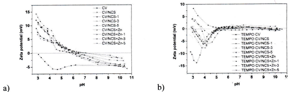
Figure 1: Zeta potential of pristine (a) and TEMPO oxidized viscose fabrics (b) functionalized with NCS and NCS+Zn before and after 1, 3 and 5 washing cycles
