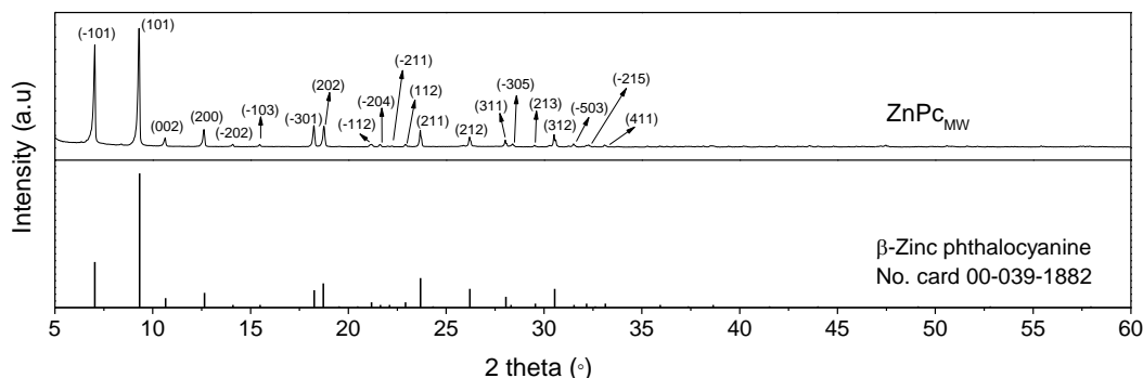
Figure 1. XRD pattern of ZnPc MW .
